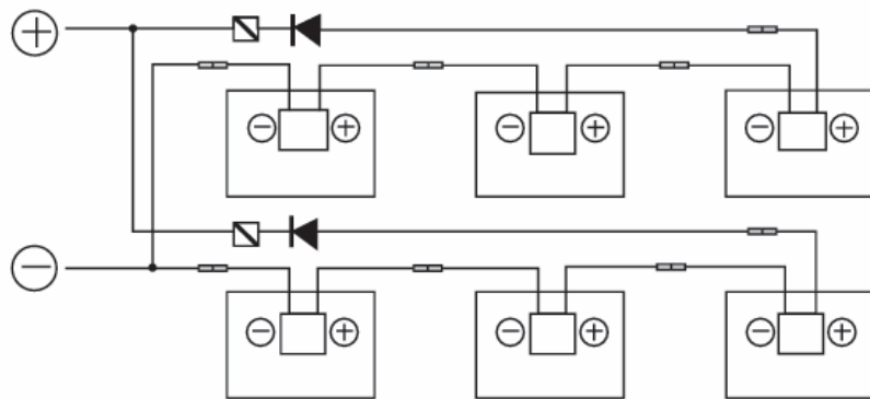
Fig. 5-5 Module connection method
